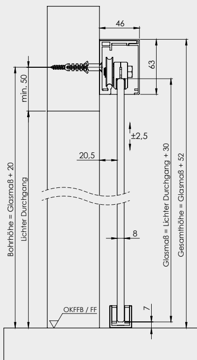
PLANEO 60 PRO, WANDMONTAGE FÜR GLASTÜREN PLANEO 60 PRO, WALL MOUNTING FOR GLASS DOORS
