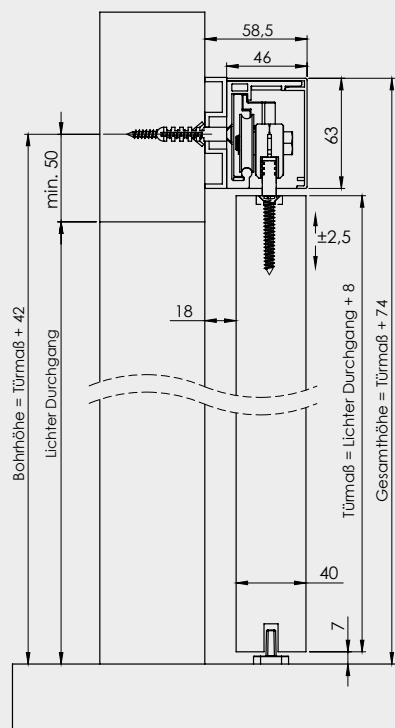
PLANEO 60 PRO, WANDMONTAGE FÜR HOLZTÜREN PLANEO 60 PRO, WALL MOUNTING FOR WOODEN DOORS
